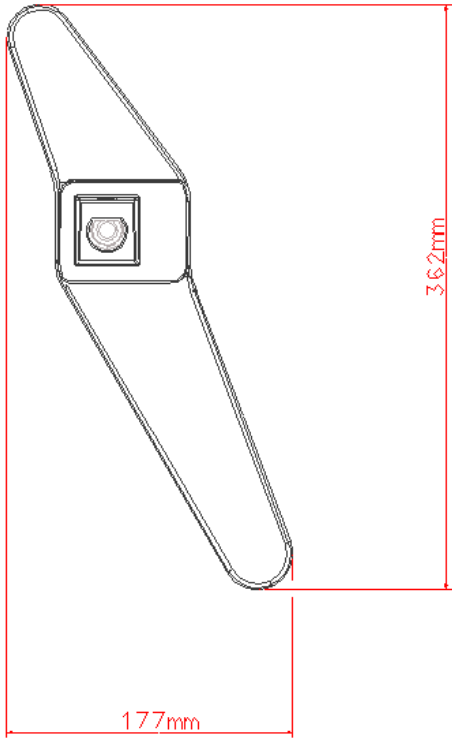
Top View
